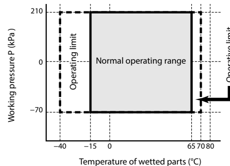
Figure 3. Working pressure and temperature of wetted parts section (for model GTX15D regular type)
