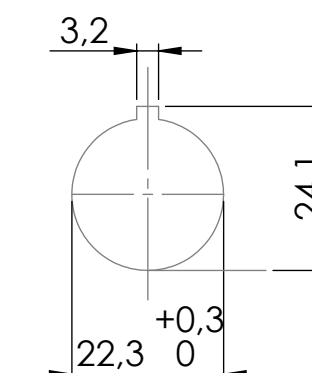
Bohrbild / Hole pattern
